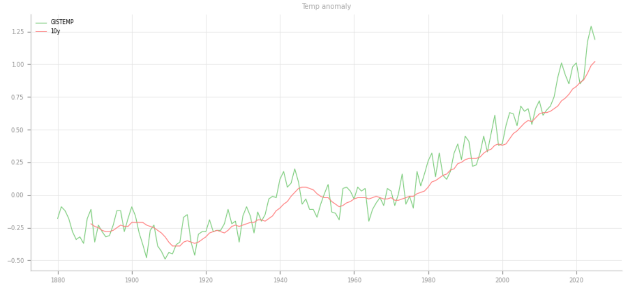
Fig. 1 – source GISTEMP
